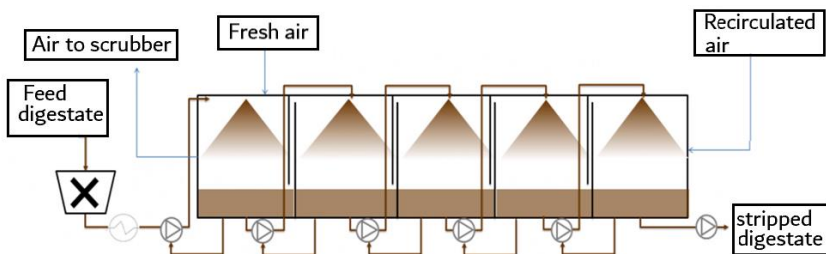
Figure 2-14 Configuration of NH_3 stripping-scrubbing on manure or digestate without packing tower. Source: AMFER, Colsen.
