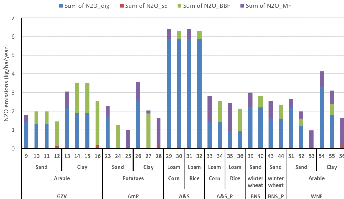
Figure 7-6 Total amounts N 2 O emissions (expressed in kg N ha -1 y -1 ) as predicted for all arable scenarios of the demonstration plants Groot Zvert Vergisting (GZV), Am-Power (AmP), Acqua & Sole (A&S), BENAS (BNS) and Waterleau NewEnergy (WNE) (mineral fertiliser is CAN).
