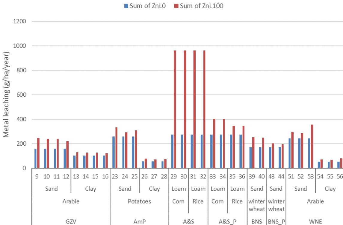
Figure 7-12 Leaching of zinc (Zn) ( \text{g ha}^{-1} \text{y}^{-1} ) for all arable crops scenarios at t=0 (ZnL0; blue bars) and after 100 years (ZnL100; red bars) for demonstration plants Groot Zvert Vergisting (GZV), Am-Power (AmP), Acqua & Sole (A&S), BENAS (BNS) and Waterleau NewEnergy (WNE).
