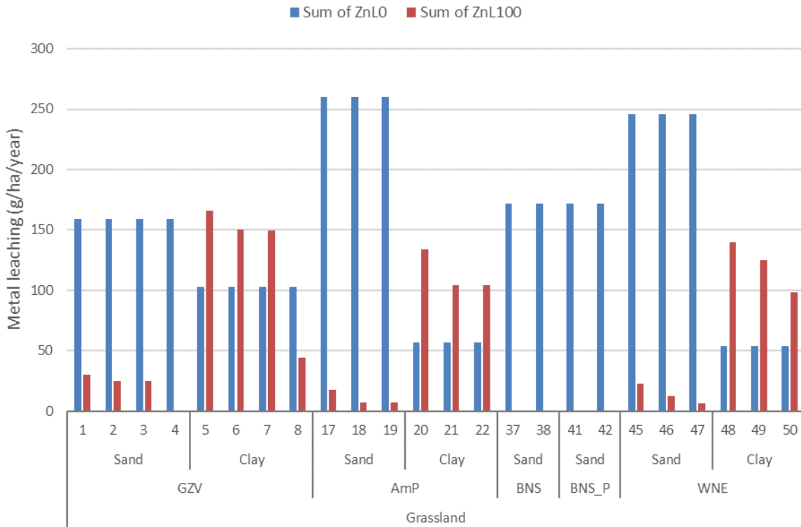
Figure 7-11 Leaching of zinc (Zn) ( \text{g ha}^{-1} \text{y}^{-1} ) for all grassland scenarios at t=0 (ZnL0; blue bars) and after 100 years (ZnL100; red bars) for demonstration plants Groot Zvert Vergisting (GZV), Am-Power (AmP), BENAS (BNS) and Waterleau NewEnergy (WNE).
