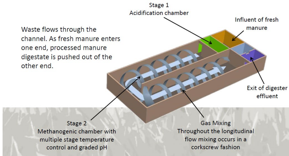
Figure 1 Process and layout of the DVO digester at Green Create
