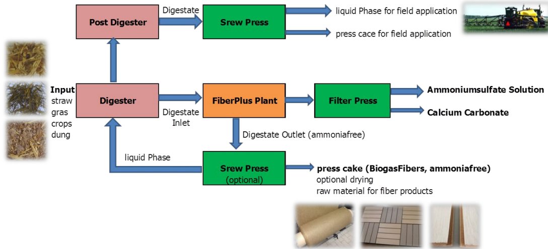
Figure 2.1: Process flows with N recovery at BENAS
