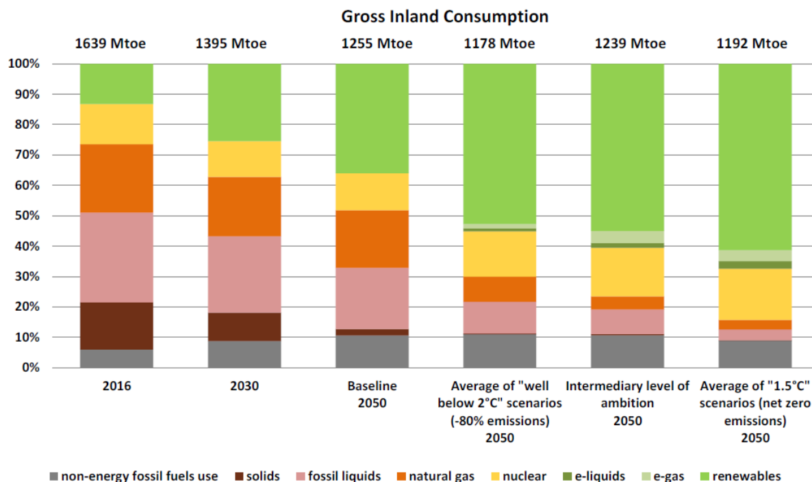
Figure 1.1 Current, 2030 and more or less ambitious 2050 energy consumption and mix scenarios (European Commission, 2018)
